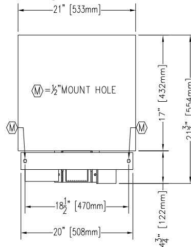
TOP FRAME
