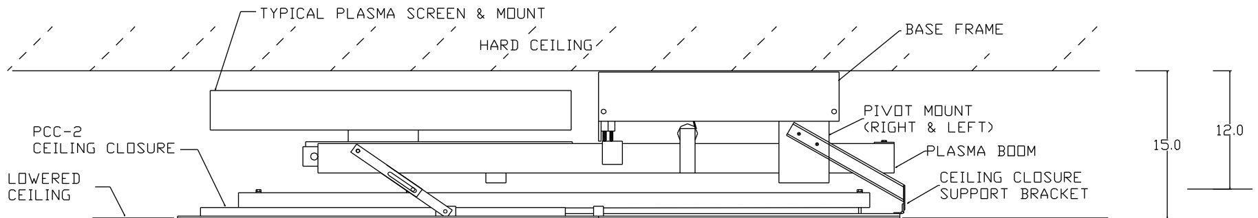
PLASMA ONE - 7 SIDE VIEW
