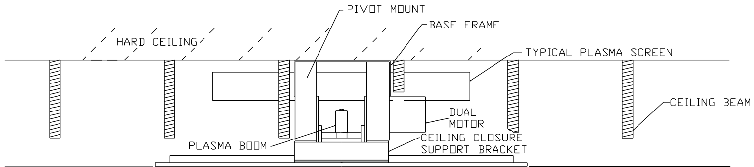
PLASMA ONE - 7 MOTOR END VIEW
